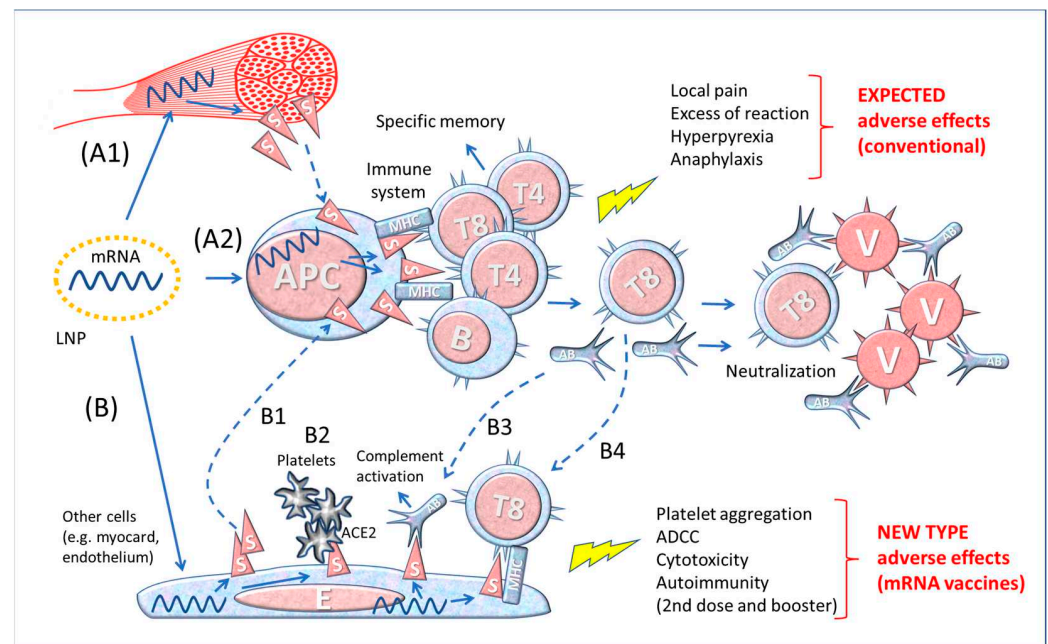
Figure 2. Diagram of the theory of functioning of anti-COVID-19 mRNA vaccines. A1–2 The simplistic theory representing the production and presentation of Spike protein by APCs to lymphocytes; A1: production of Spike by local muscle cells and release (by shedding) of soluble S that would be captured and processed by APC for immune stimulation; A2: the LNPs transfect the mRNA into APCs, which then produce and present in the context of MHC Spike to immune cells. B. Theoretical consequences of the expression of Spike protein by cell types other than immune cells transfected by mRNA containing LNP. B1: S protein released by somatic cells stimulates the immune system via APC; B2: interaction of blood platelets with S protein on the membrane of endothelial cells; B3: specific antibodies bind to S protein on the membrane of somatic cells (myocardium, endothelium, etc.) and activate the Complement system (or antibody-dependent cytotoxicity; not shown) leading to cell death; B4: specific CD8+ T lymphocytes (T8) attack endothelial cells expressing S protein. Abbreviations and symbols: LNP: lipid nanoparticle; APC: antigen-presenting cell; MHC: Major Histocompatibility Complex; S: Spike; T and B: lymphocytes; V: Virus; E: Endothelial cell; AB: Antibody; ADCC: Antibody-dependent cell cytotoxicity; ACE2: angiotensin-converting enzyme 2. Solid line arrows: action, operation; dashed line arrows: moving, displacement.
