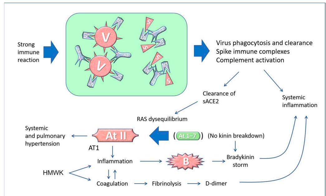
Figure 4. Pathological effects of COVID-19 and the vaccine on the renin-angiotesin system (the balance between angiotensin II and angiotensin 1–7 is illustrated here). ACE2 normally destroys angiotensin II, an 8-amino acid peptide that has a hypertensive action and causes water retention, and converts it into “angiotensin 1–7”, which has a hypotensive effect. Abbreviations and symbols: RAS: Renin-angiotesin system; E: Endothelial cell; V: Virus; S: Spike; A: ACE2; sA: soluble ACE2; ATII: Angiotensin II; At 1–7: Angiotensin 1–7; B: Bradykinin; Ab: Antibody; HMWK: High molecular weight kininogen; AT1: Angiotensin II receptor type 1.
