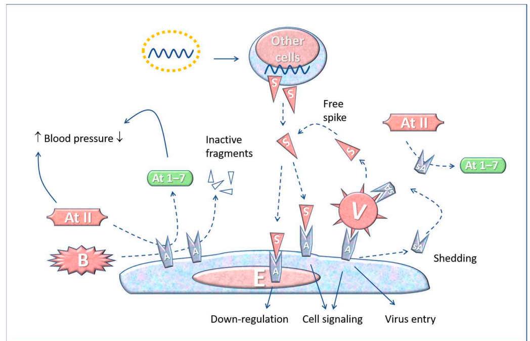
Figure 3. The interaction between SARS-CoV-2 and free Spike protein with ACE2 receptors on the membrane of an endothelial cell. The interaction favours the virus entering the cell (e.g., platelets, leucocytes, macrophages, endothelia) as well as the cell activation by the free Spike. ACE2 can convert angiotensin II (made from 8 amino acids) into an inactive form (1–7), and can inactivate bradykinin, a major mediator of acute inflammation. The Spike–ACE2 interaction can lead to platelet aggregation, inflammation and thrombosis, as described in the text. Abbreviations and symbols: E: Endothelial cell; V: Virus; S: Spike; A: ACE2; sA: soluble ACE2; ATII: angiotensin II; At 1–7: angiotensin 1–7; B: Bradykinin. Solid line arrows: action, operation, effect; dashed line arrows: moving, conversion.
