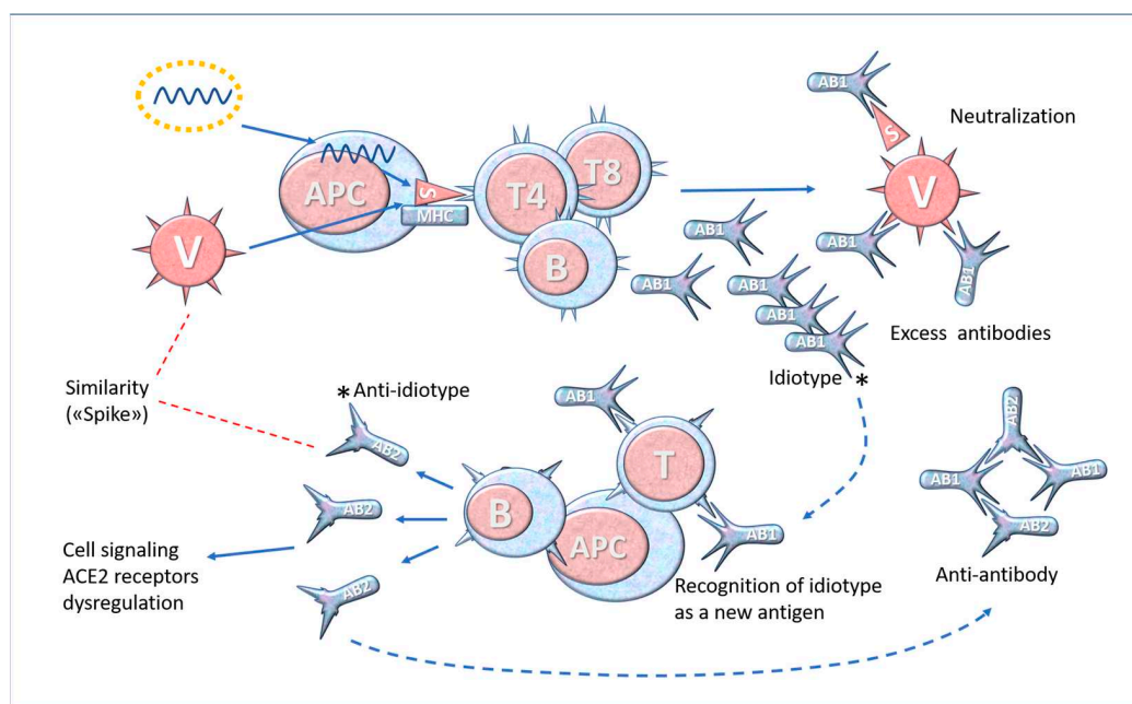
Figure 6. Simplified diagram of anti-idiotype antibody formation. A variable part of the antibody (Ab1) able to bind to the Spike is called idiotype. Since this part is a “new” protein within the repertoire of antigens known to the immune system, the latter produces antibodies (Ab2) in response to the idiotype, which can recognise and bind to it. These secondary antibodies, called “anti-idiotype”, represent in a certain way the internal image of the external antigen (Spike) and may share some of its biological properties. * Molecular complementarity of idiotypes.
